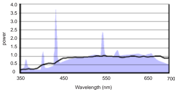
Spectral Power Distribution Graphiclite 100 D50 Lamp
