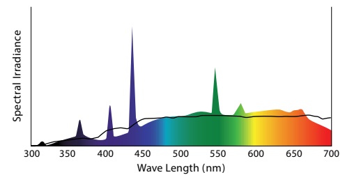
Figure 3. High CRI, 5000K Graphilite Fluorescent
